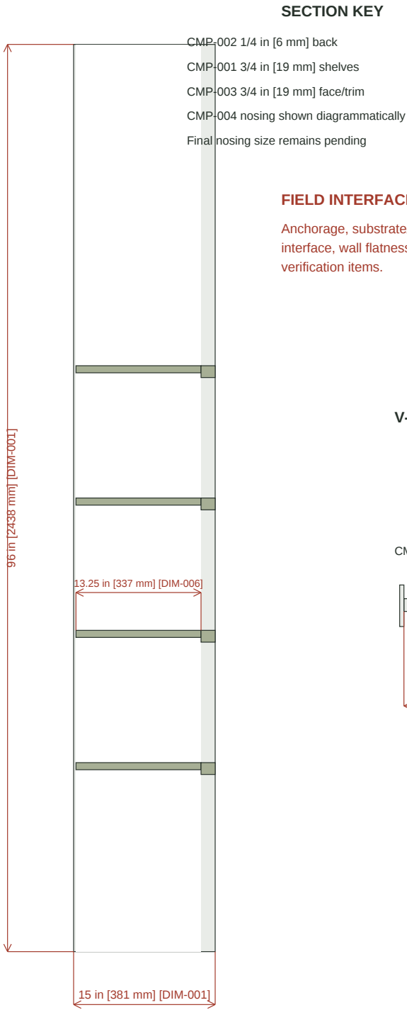
V-A102-02 CENTER-BAY VERTICAL SECTION
