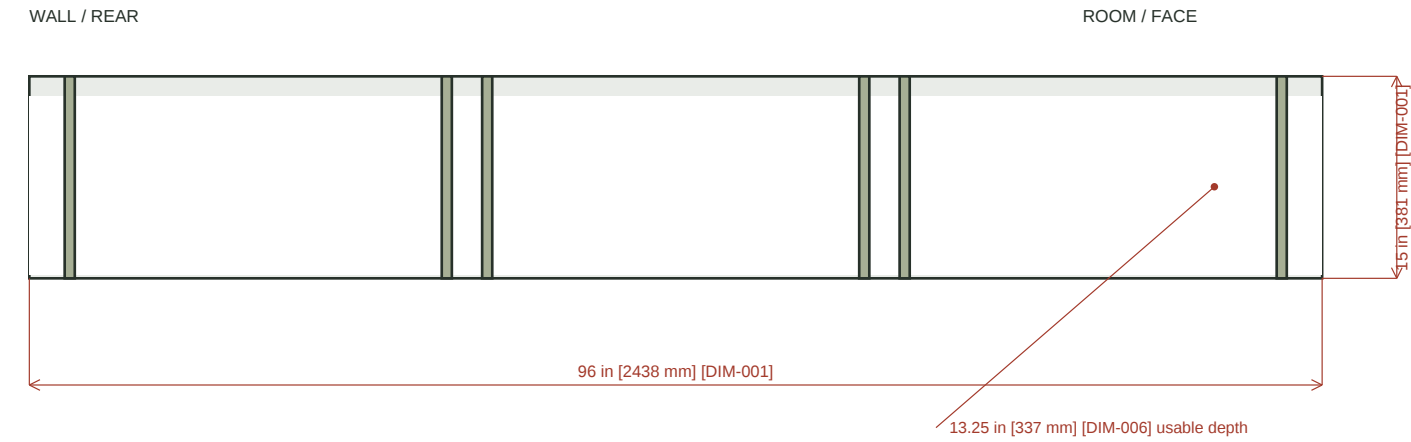
V-A102-01 HORIZONTAL / DEPTH SECTION
